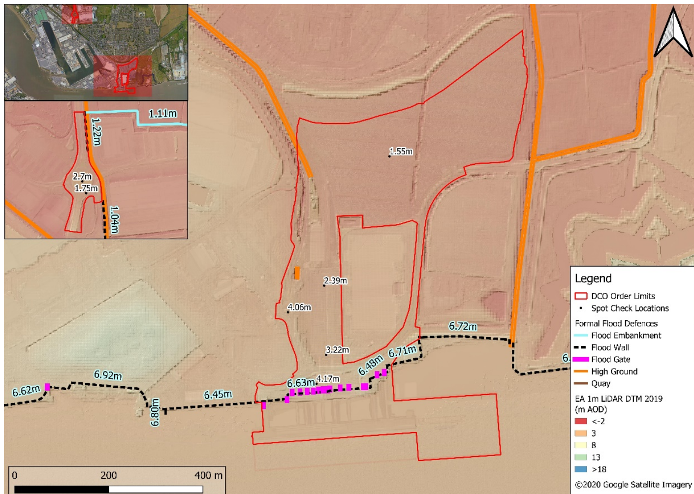
Figure 17.3: Existing flood defence alignment and crest levels taken from EA data and spot elevations of existing land levels taken from LiDAR 2019 for the Essex Project Site.
